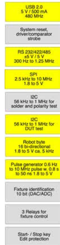
Multifunction board
