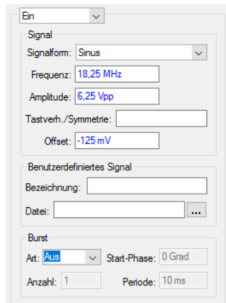
Curve form editor of the function- and arbitrary generator
